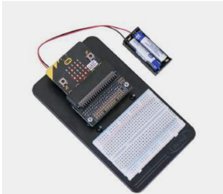
Kitronik Prototyping System for the BBC micro:bit
