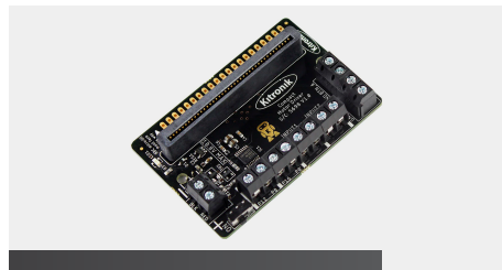
Kitronik Compact Motor Driver Board for the BBC micro:bit SKU: 204-8223 MPN: 5698
