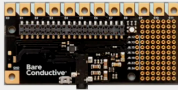
Bare Conductive Pi Cap SKU: 189-4512 MPN: SKU-6515
