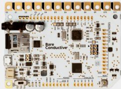
Bare Conductive Touch Board SKU: 837-1729 MPN: SKU-5006
