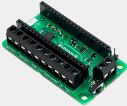
Kitronik Motor Driver Board for Raspberry Pi Pico SKU: 224-7772 MPN: 5331
