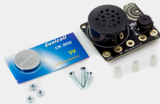
Kitronik MI:sound speaker board for BBC microbit V2 SKU: 217-6976 MPN: 5649-V2
