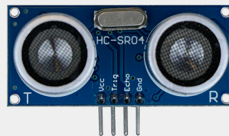
Ultrasonic Distance Sensor HC-SR04 5V Version SKU: 215-3181 MPN: 46130
