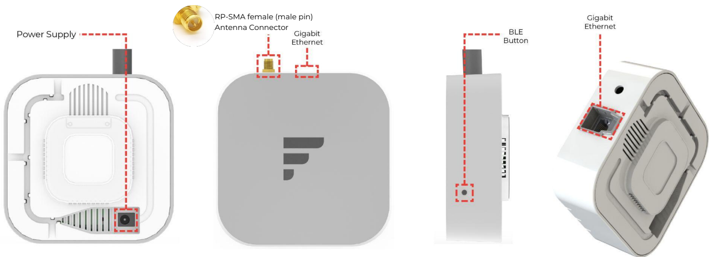
Figure 3: FinestraMiner Interfaces
