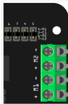
Fig4: PWM Motor Control Pin Allocation
