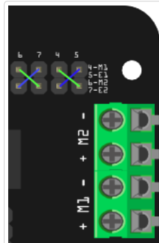
Fig5: PLL Motor Control Pin Allocation Configuration
