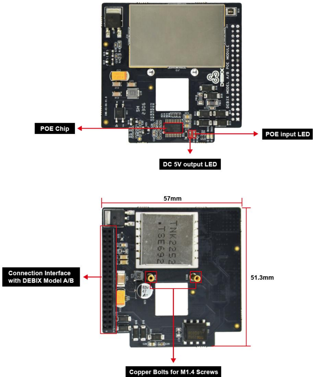
Figure 2 DEBIX POE Module
