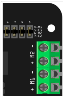
(/wiki/index.php/File Fig4: PWM Motor Control Pin Allocation
